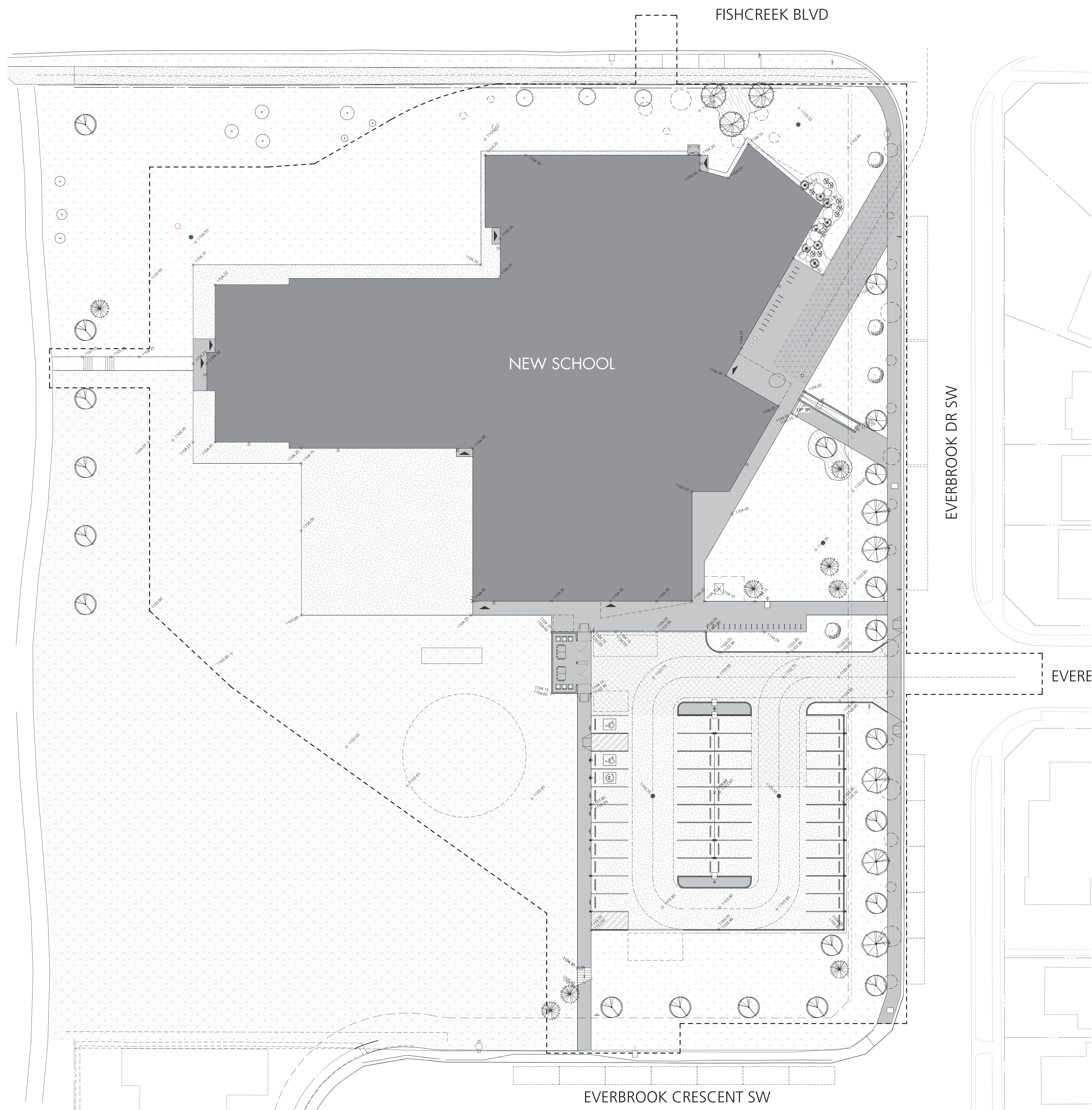
PROPOSED SITE PLAN NTS
