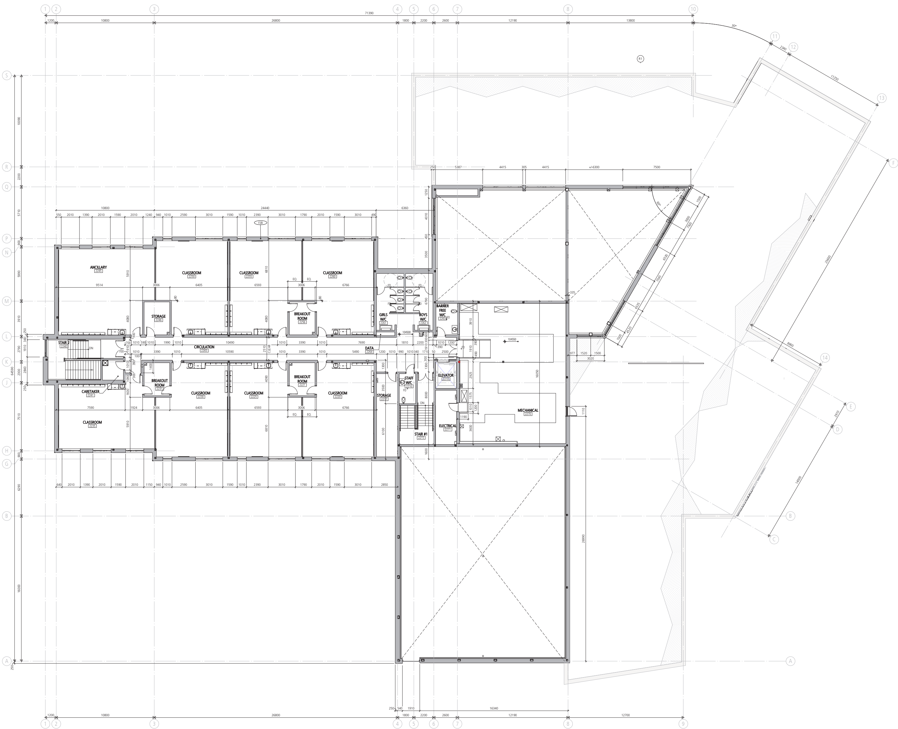
1 SECOND FLOOR PLAN NTS
