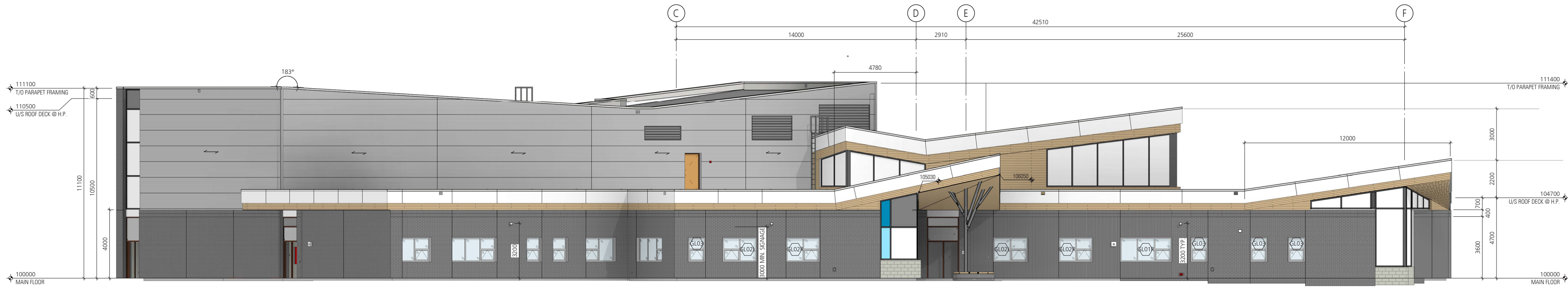
EAST ELEVATION
