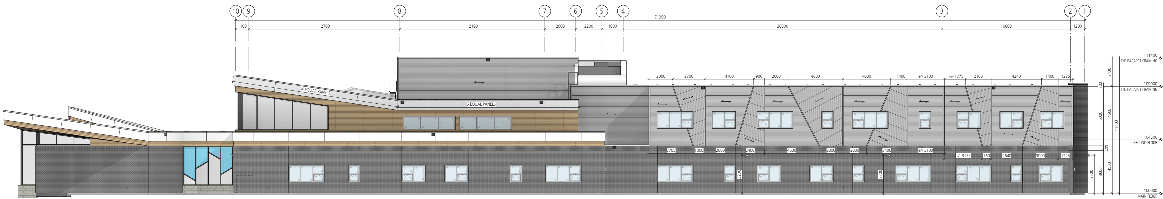
NORTH ELEVATION
