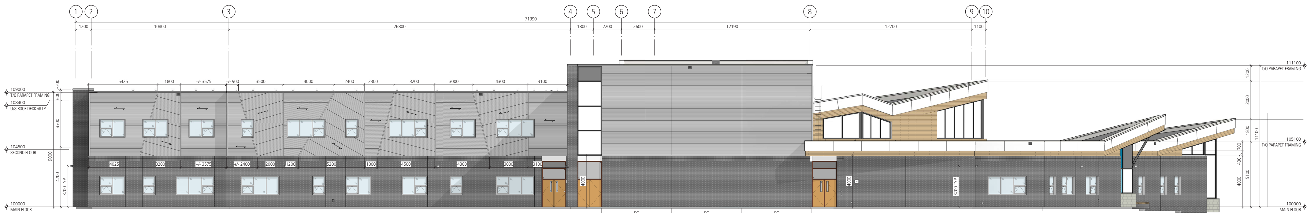
SOUTH ELEVATION
