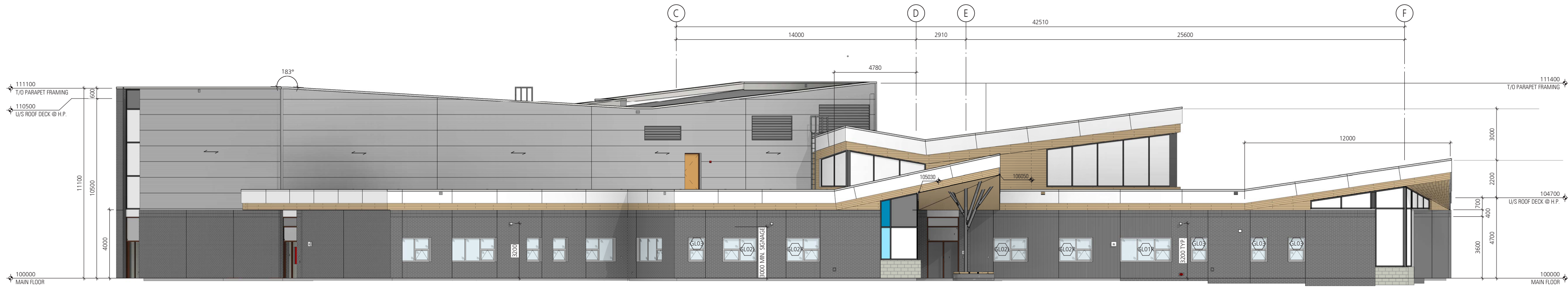
SOUTH ELEVATION
