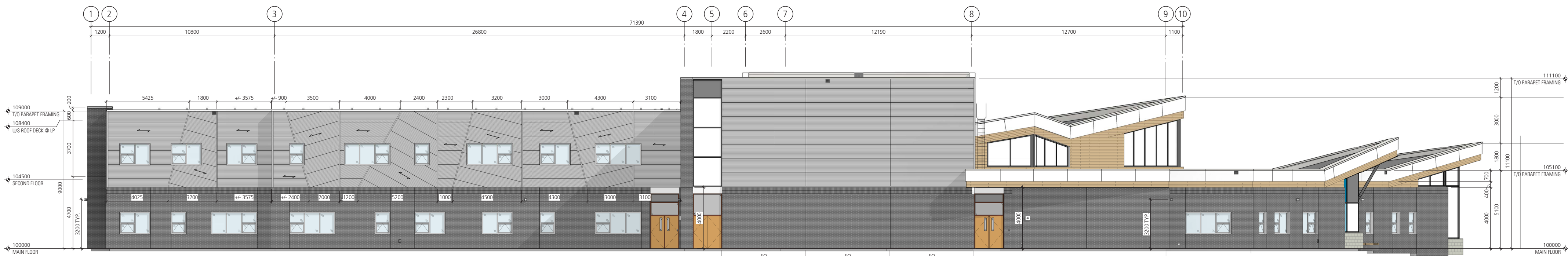
WEST ELEVATION
