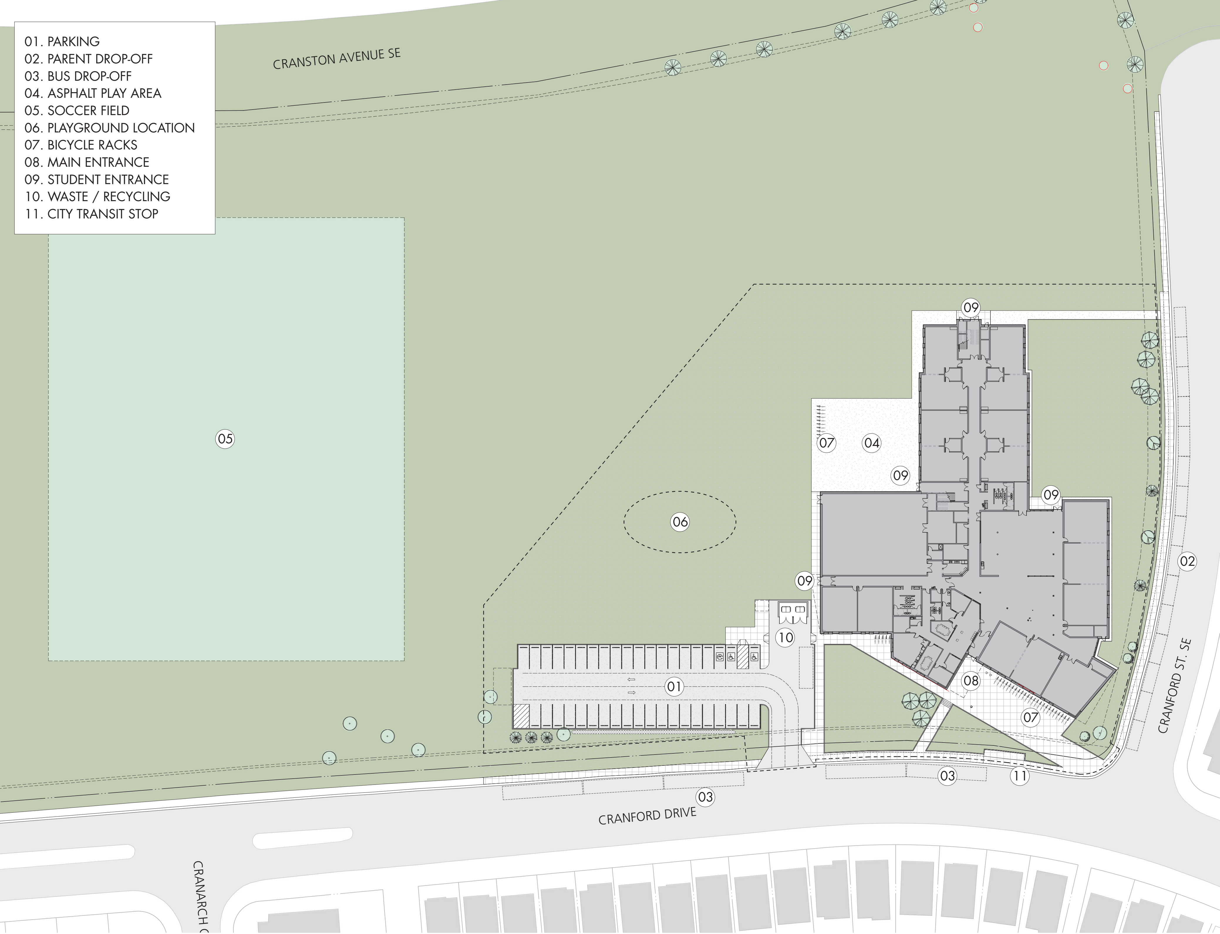
1 PROPOSED SITE PLAN
